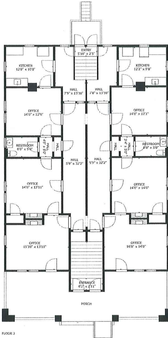
FLOOR 2
