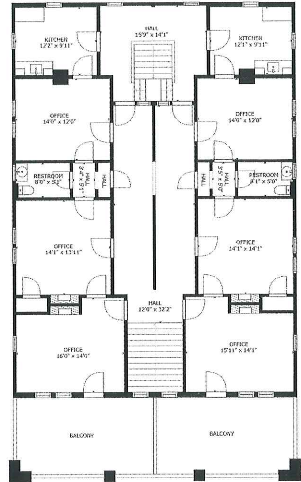
FLOOR 3
